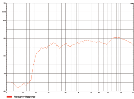
⊙ Artist T3频响曲线图
