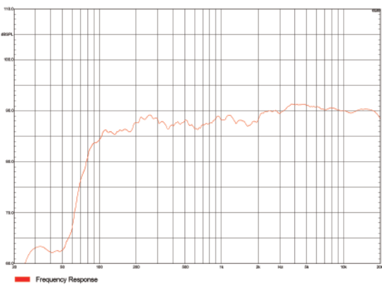
⊙ Artist T4频响曲线图
