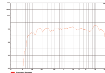
Artist T83 Frequency Response Curve
