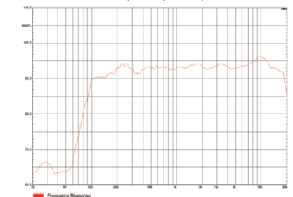
Artist T43 Frequency Response Curve
