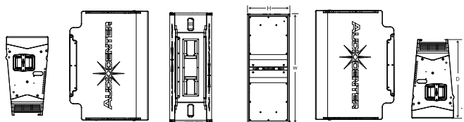
Dimension(WxHxD): 899x344.5x647.5mm
