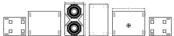
Dimension(W×H×D): 1080×595×760mm
