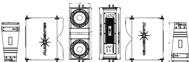
尺寸(WxHxD):590x236x500mm
